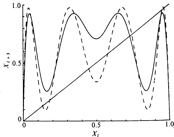
Fig. 5 The relationship between X_{i+3} and X_i , obtained by three iterations of equation (3). The solid curve is for a = 3.7 , and only intersects the 45° line once. As a increases, the hills and valleys become more pronounced. The dashed curve is for a = 3.9 , and six new period 3 points have appeared (arranged as two cycles, each of period 3).
